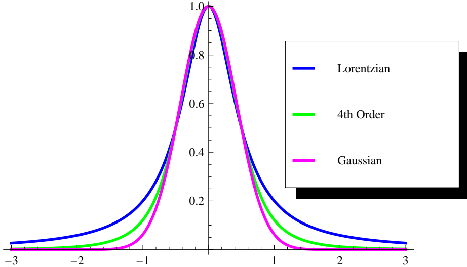
Figure 9: Lorentzian, Intermediate (4th Order) and Gaussian Pulses
