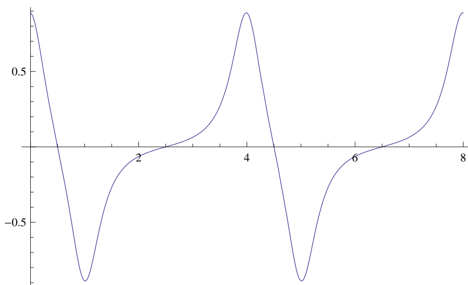
Figure 2: Simple Dibit Test Pattern
